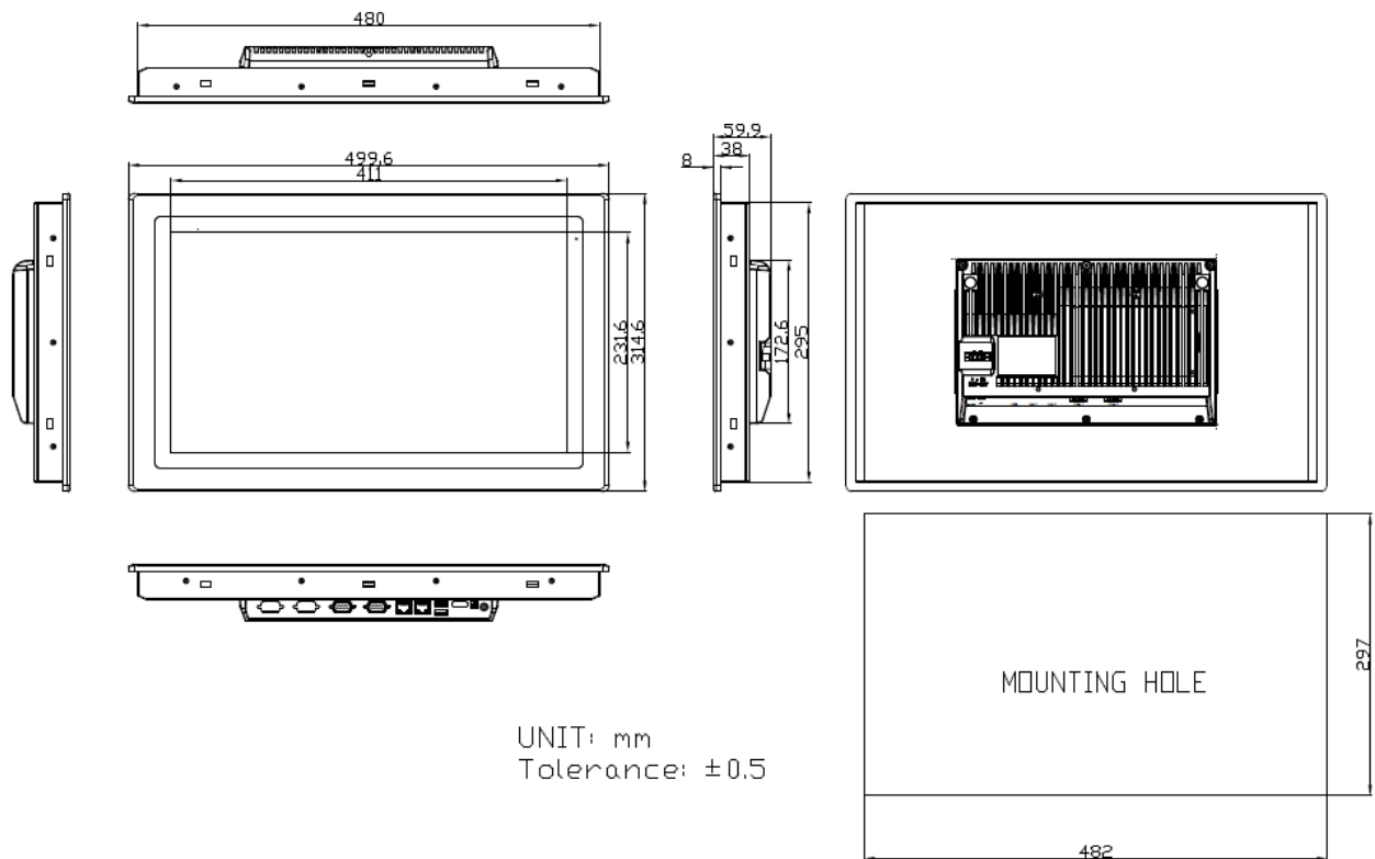
Figure 1.8: Dimensions of ARCHMI-818(P)
