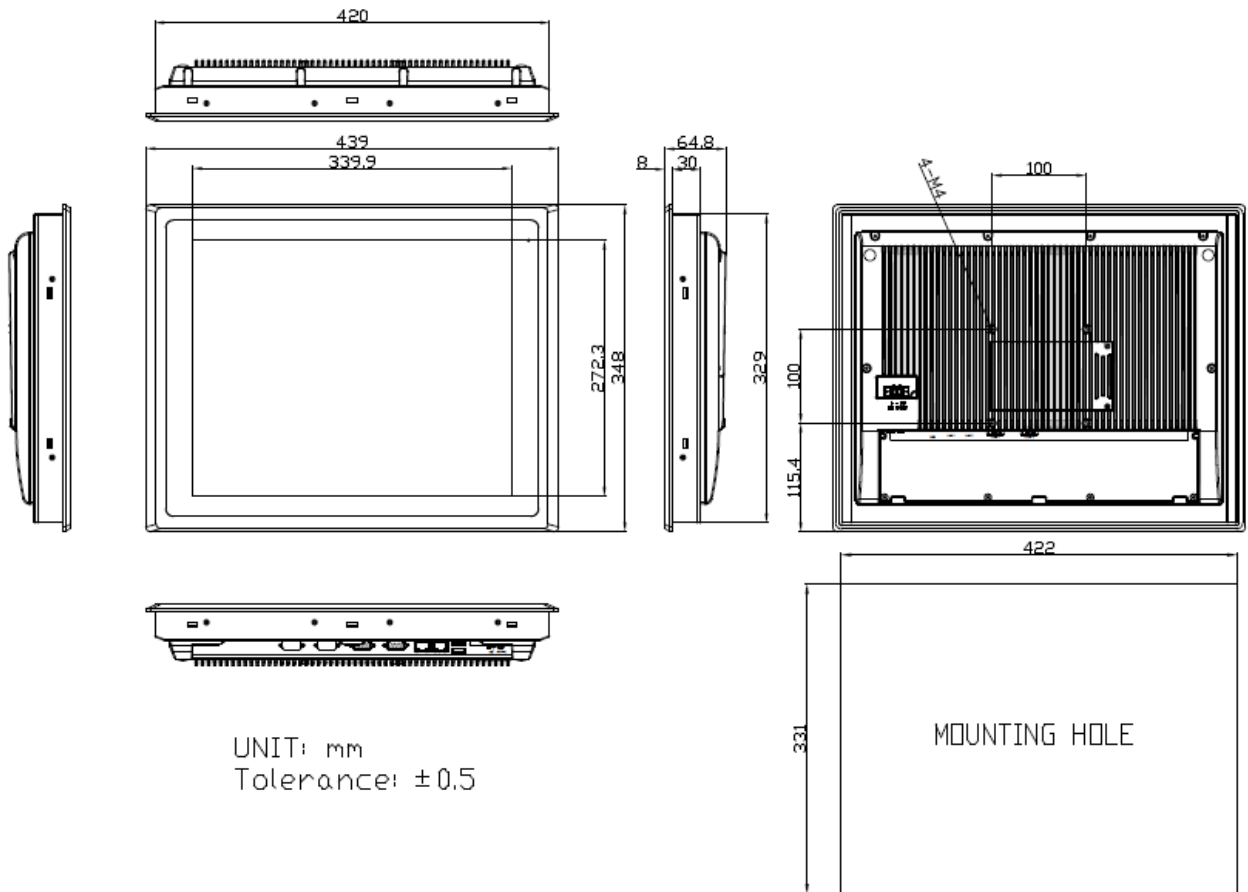
Figure 1.7: Dimensions of ARCHMI-817(P)
