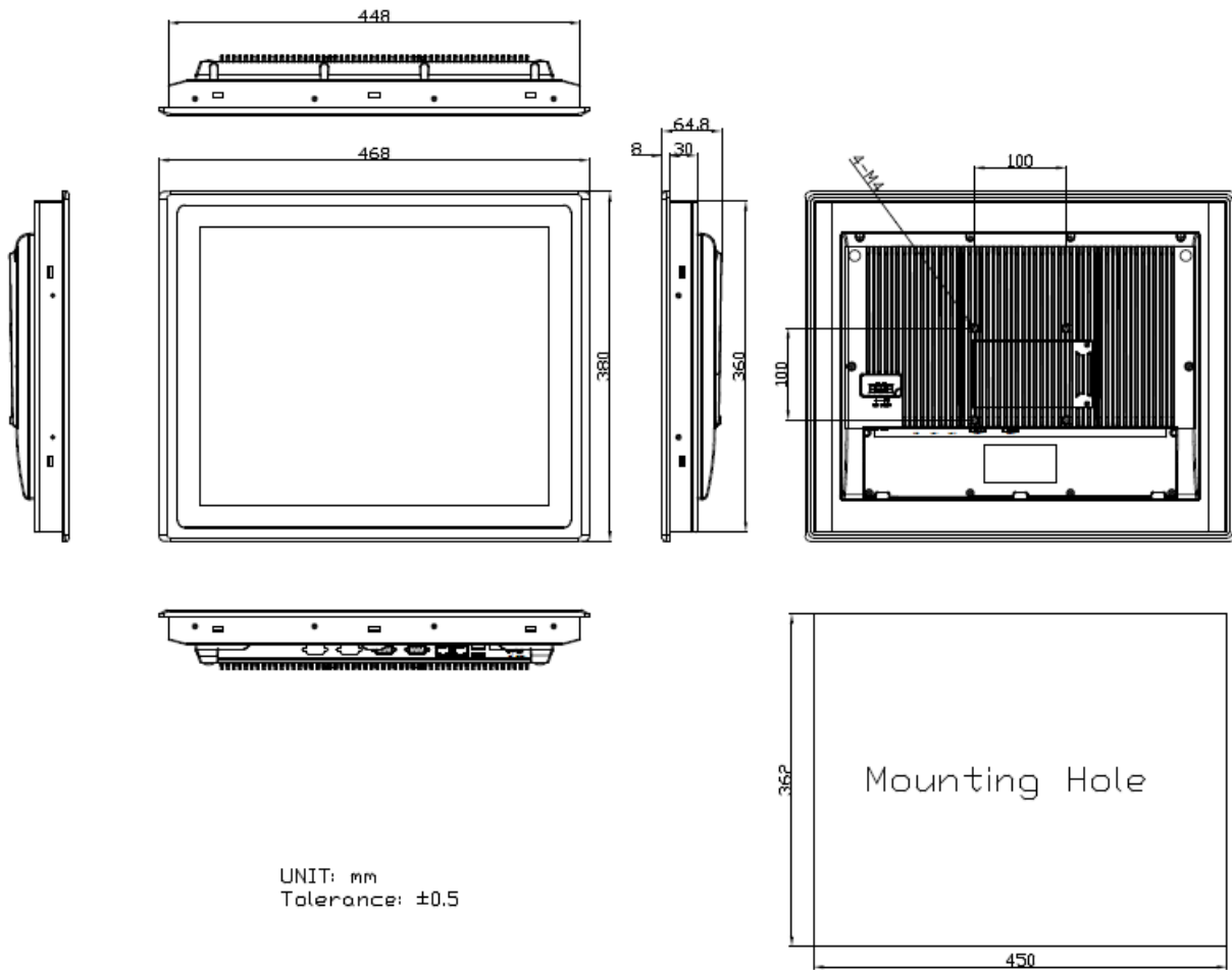
Figure 1.9: Dimensions of ARCHMI-819(P)
