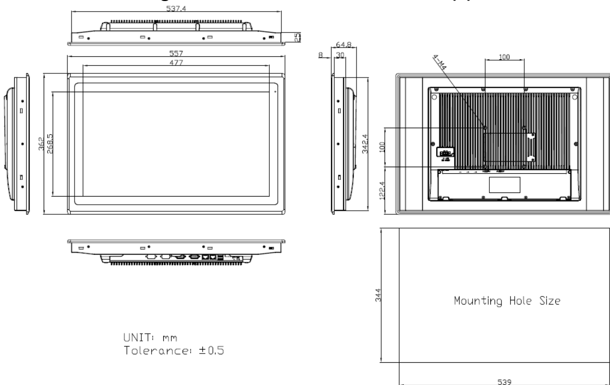
Figure 1.10: Dimensions of ARCHMI-821 (Resistive Touch)
