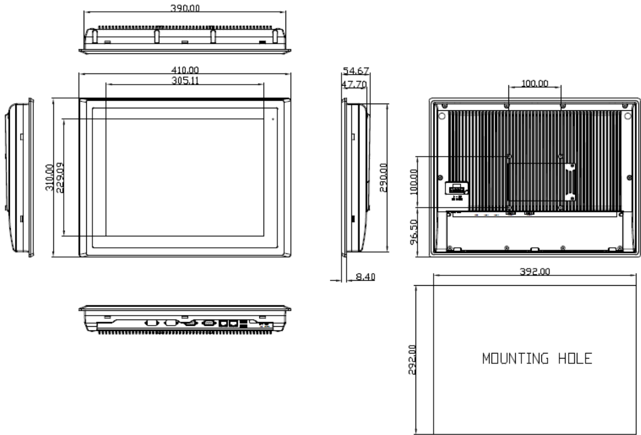
Figure 1.5: Dimensions of ARCHMI-815(P)
